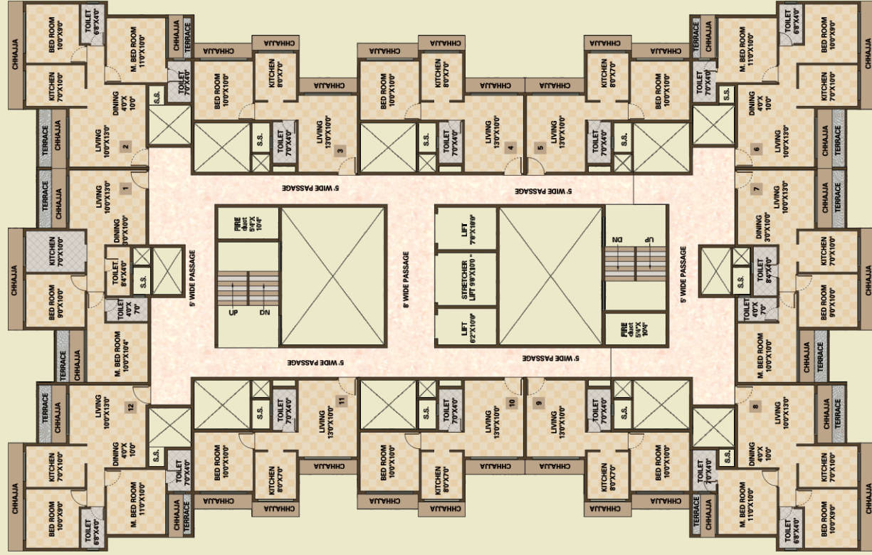
4th, 6th & 8th FLOOR PLAN
