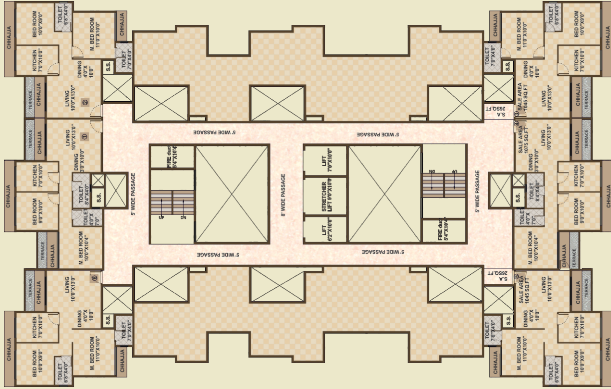
10th To 14th FLOOR PLAN
